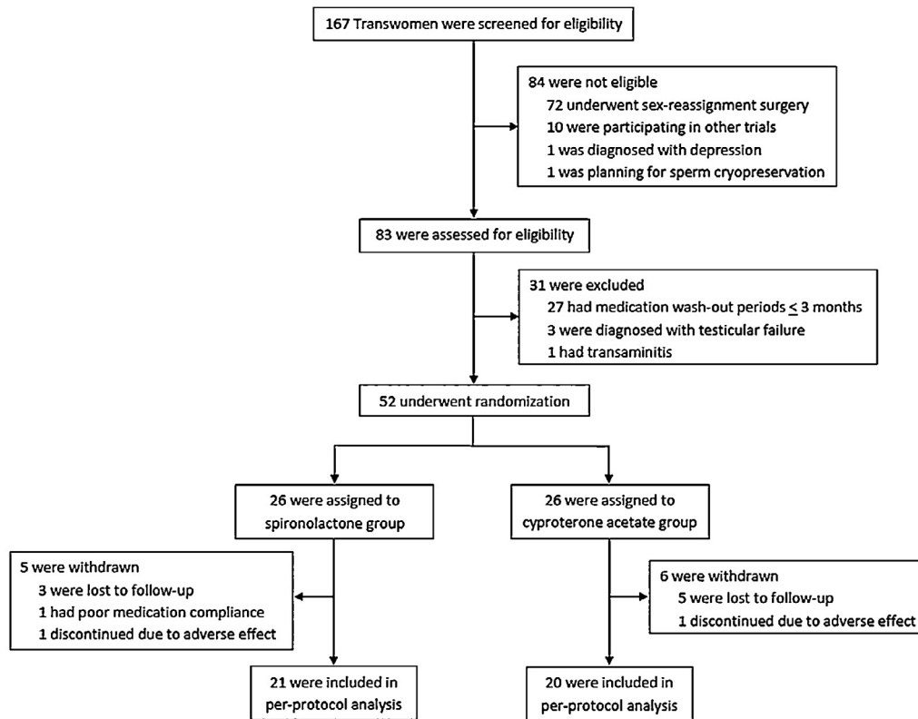
Figure 1. Study flow.
